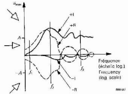
FIG. 9c. — Spectres tracés pour un nombre infini de fréquences, f_1 , f_2 et f_3 étant des points finis de la courbe continue. Spectra which result from an infinite number of frequencies, with f_1 , f_2 and f_3 shown as finite points on the continuous curves.
