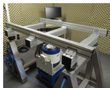
m series shakers (SAREX-UNO) Compact and Low Acoustic Noise Vibration Test Systems
